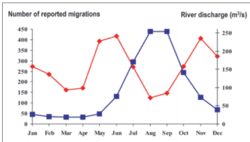
Figure 5: Relationship between migratory activity levels and water discharge in the Lower Mekong Basin (modified from Bouakhamvongsa and Poulsen, 2000) Blue Line: average monthly discharge ( \text{m}^3/\text{sec} ) of the Mekong River at Pakse, Southern Lao PDR (data provided by MRC Secretariat). Red Line: Number of migration reports (based on 50 species from 51 sites along the Mekong mainstream).
