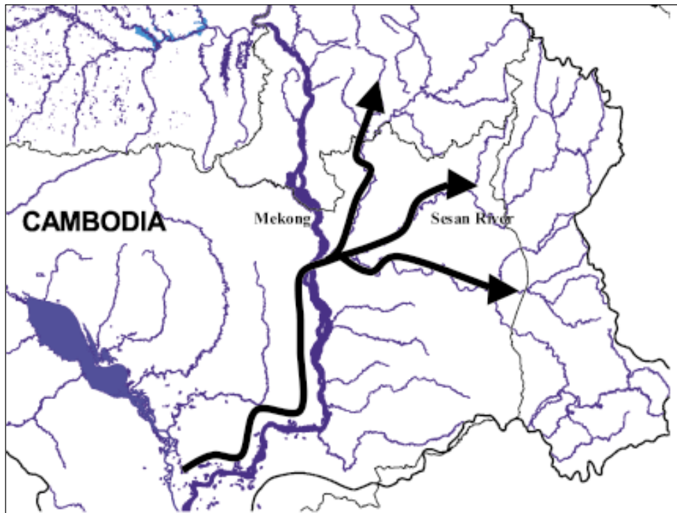
Figure 7: The dry-season migration of Henicorhynchus spp. from the Mekong into the Sesan Tributary system
